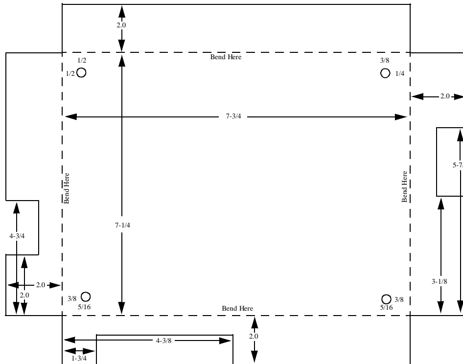
EFI 4-Layer Case Cut Pattern (Bottom) Bold Lines are Cut, Dotted Lines are Bent Up Dimension Assumes use of 1/2" Board Spacers All Dimensions in Inches
